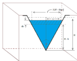
Gambar 2.1 Weir V Notch 90° (Salam,2021)
