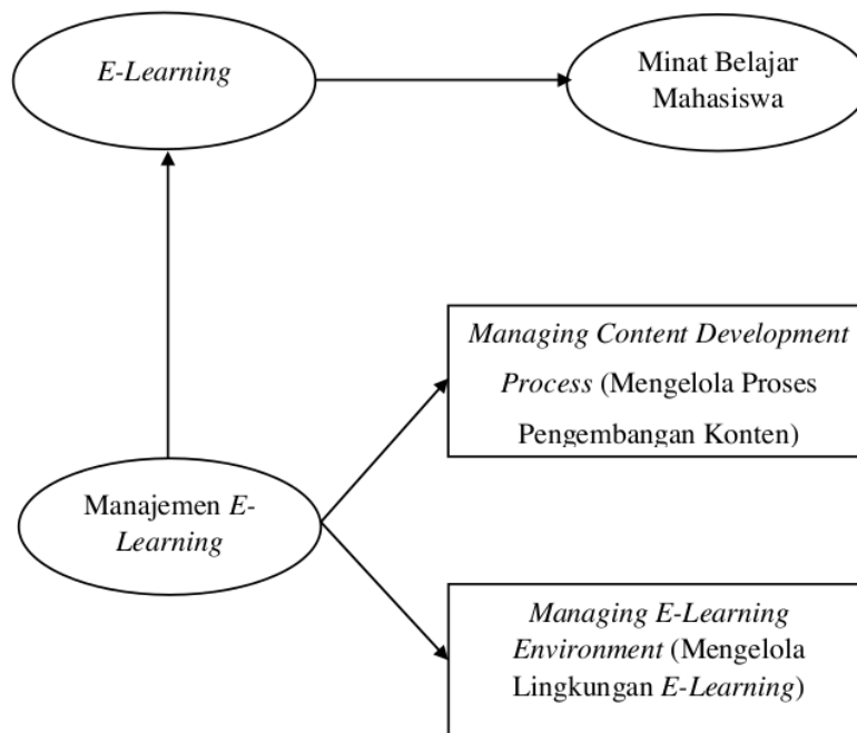
Gambar 1. Conceptual Framework
