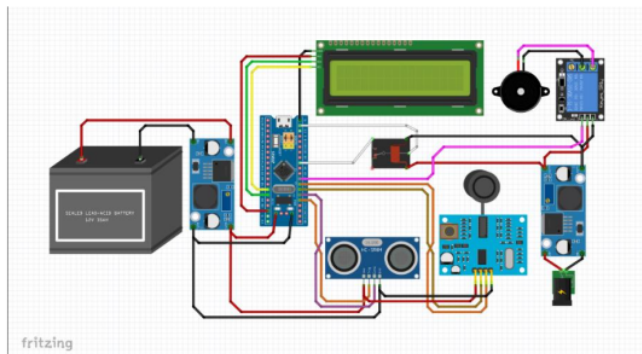
Gambar 4. Setting Peralatan Penelitian
