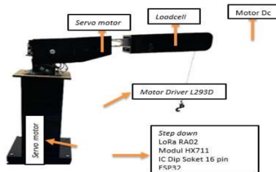
Gambar 4. 9 Perakitan prototype Crane
