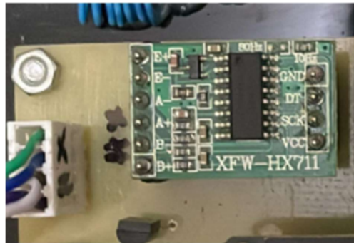
Gambar 4. 3 Sensor modul HX711
