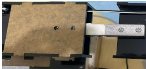
Gambar 4. 2 sensor Loadcell
