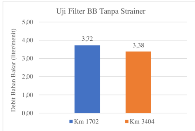
Gambar 3. Uji Filter Tanpa Strainer
