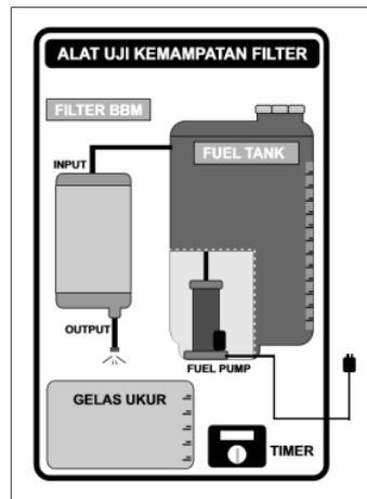
Gambar 1. Setting Peralatan Penelitian
