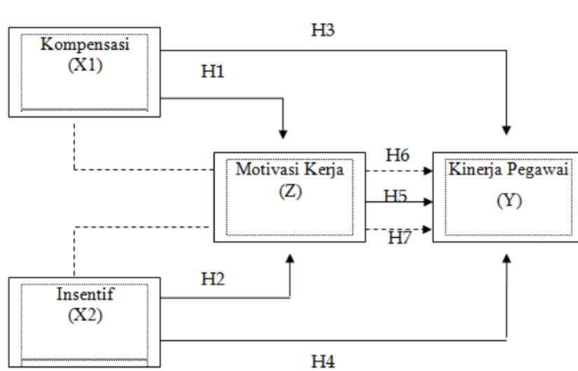
Gambar 1. Conceptual Framework
