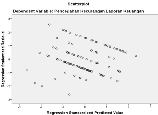
Gambar 1. Scatterplots
