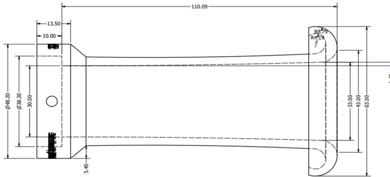
Gambar 6 Velocity Stack 110 mm
