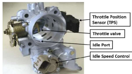
Gambar 1 Throttle Body
