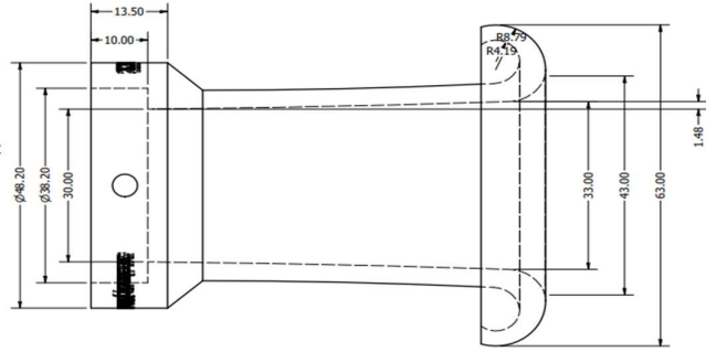
Gambar 5 Velocity Stack 70 mm
