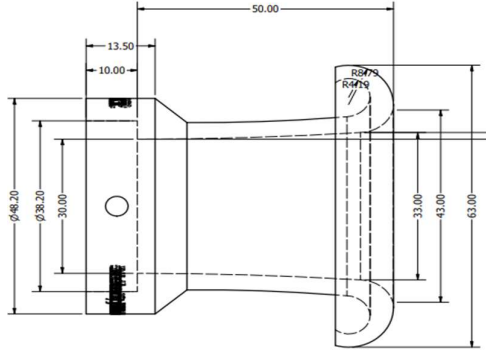
Gambar 4 Velocity Stack 50 mm
