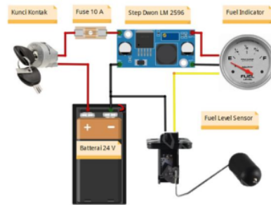
Gambar 4. Setting Peralatan Penelitian
