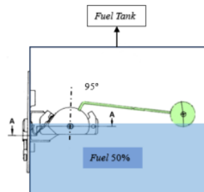
Gambar 9. Skematik Fuel Level Sensor Sudut 95°
