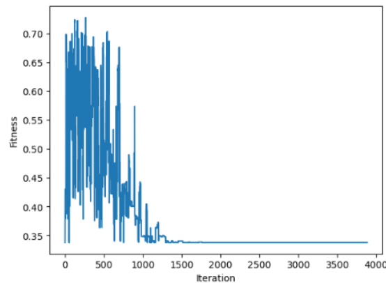
Gambar 6. 2 Hasil fitness Simulated Annealing
