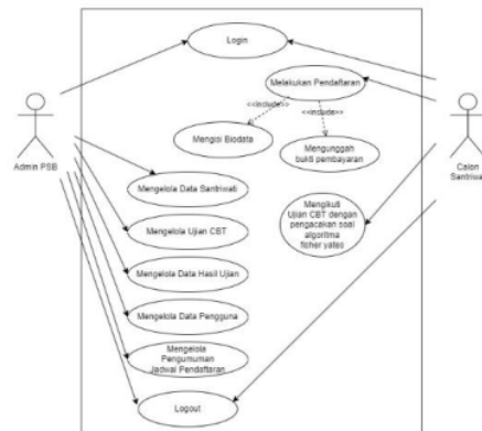
Gambar 1 Usecase Diagram
