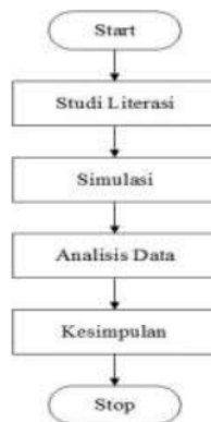
Gambar 2. Alur Penelitian
