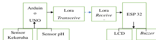
Gambar 10 Blok diagram
