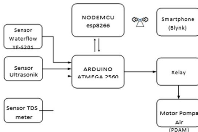
Gambar 1 Blok diagram hardware
